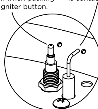
Igniter Housing removed for visibility
