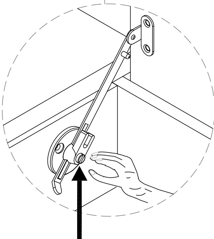
Friction screw
