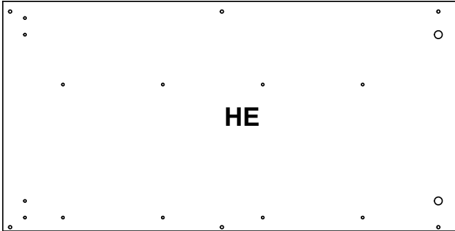
871x442x15mm
