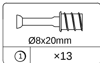
CAM BOLT TGO 2000
